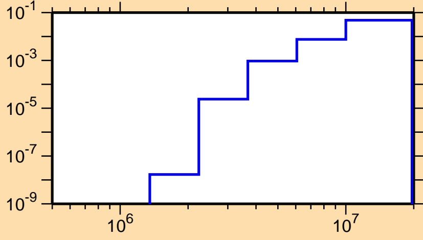
\sigma vs. E for ^{58}\text{Cu}(n,d)
