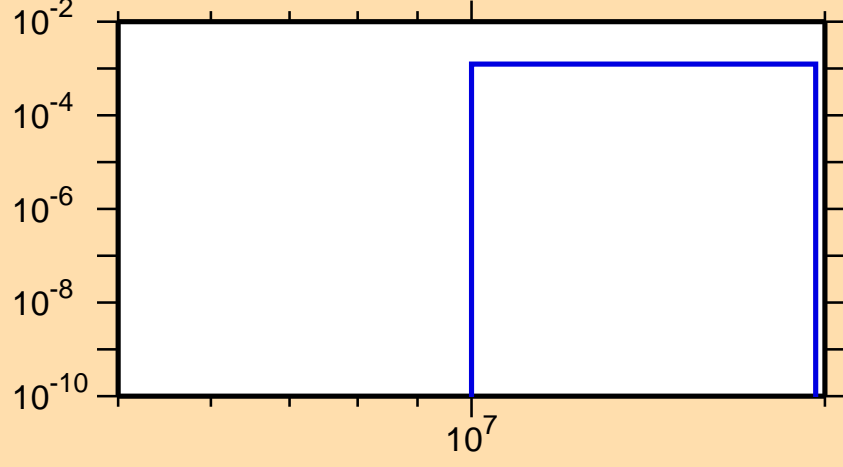
\sigma vs. E for ^{58}\text{Cu}(n,pd)
