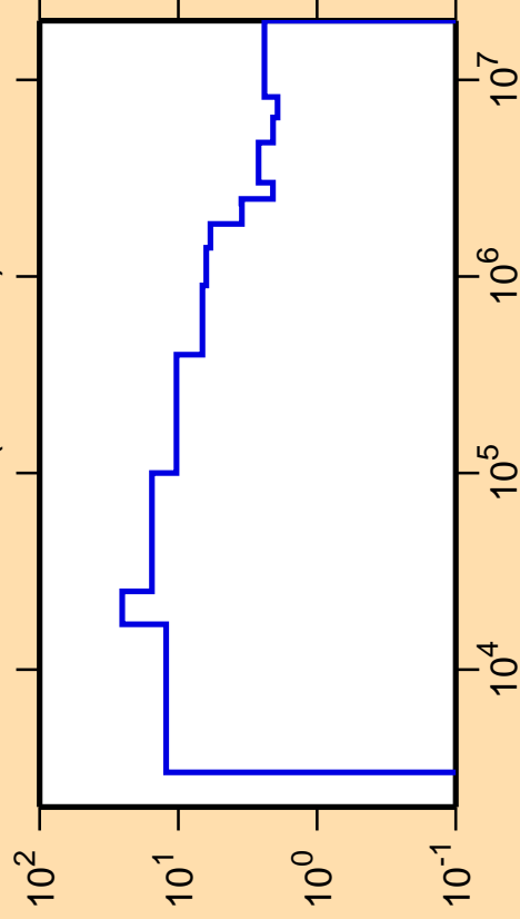
\Delta\sigma/\sigma vs. E for ^{58}\text{Cu}(n,\text{nonel.})
