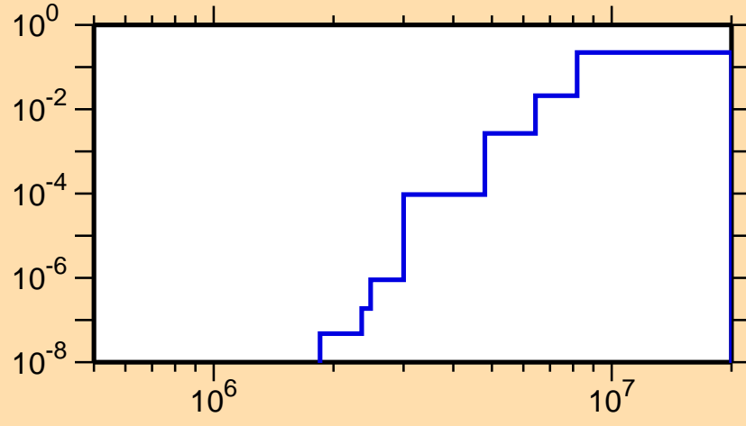
\sigma vs. E for ^{58}\text{Cu}(n,p\alpha)
