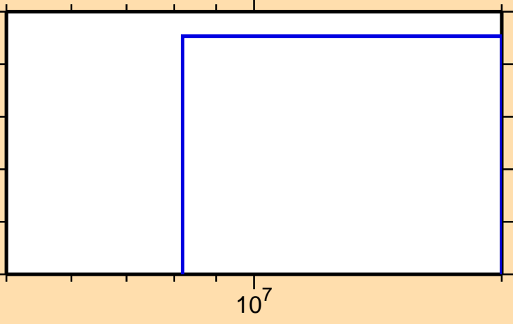
\sigma vs. E for ^{58}\text{Cu}(n,2np)
