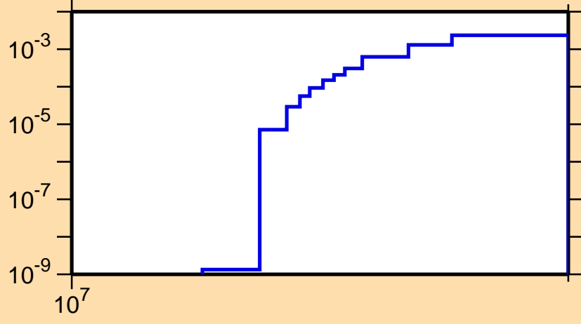
\sigma vs. E for ^{59}\text{Cu}(n,2n)
