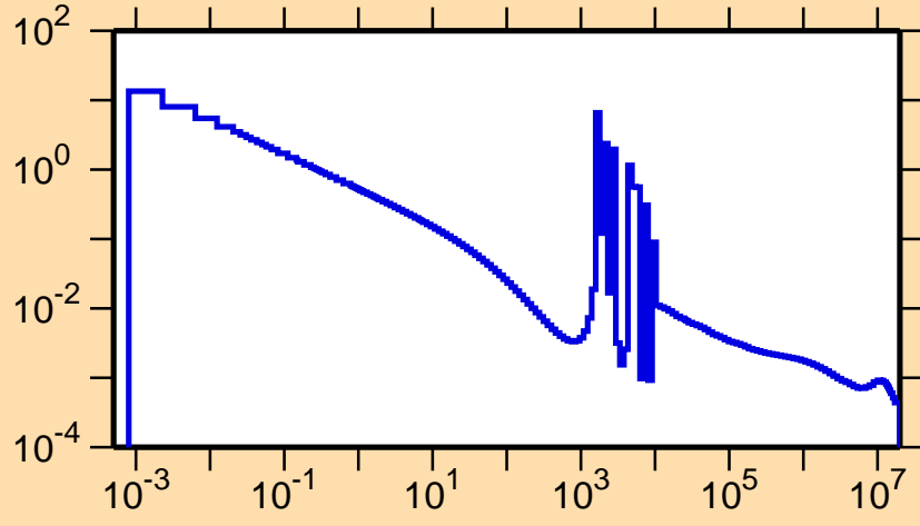
\sigma vs. E for ^{59}\text{Cu}(n,\gamma)
