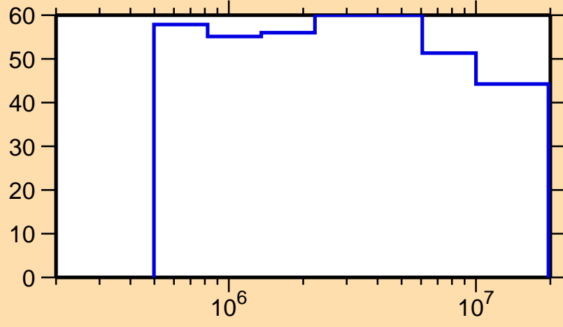
\Delta\sigma/\sigma vs. E for ^{59}\text{Cu}(n,n_1)
