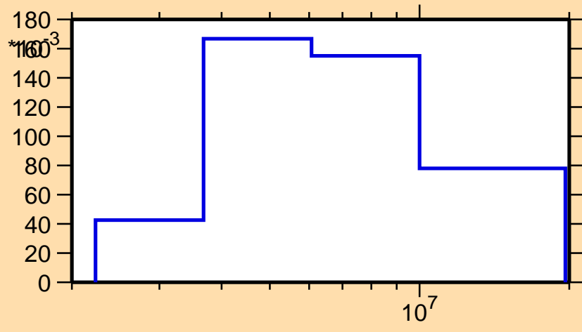
\sigma vs. E for ^{59}\text{Cu}(n,n\text{cont.})
