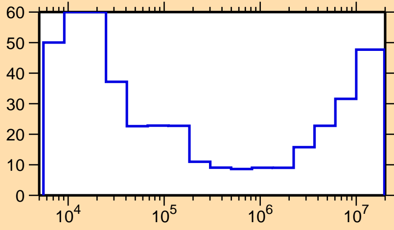
\Delta\sigma/\sigma vs. E for ^{59}\text{Cu}(n,p)
