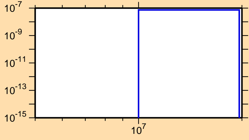
\sigma vs. E for ^{59}\text{Cu}(\text{mt117})
