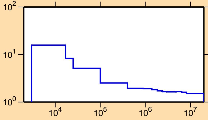
\sigma vs. E for ^{59}\text{Cu}(n,\text{nonel.})
