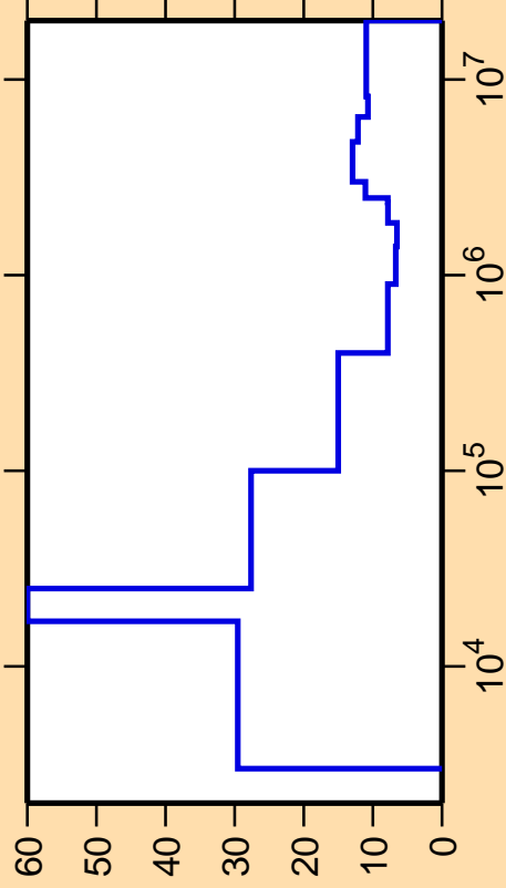
\Delta\sigma/\sigma vs. E for ^{59}\text{Cu}(n,\text{nonel.})
