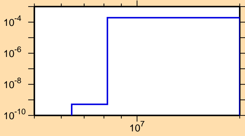
\sigma vs. E for ^{59}\text{Cu}(n,\text{He}3)
