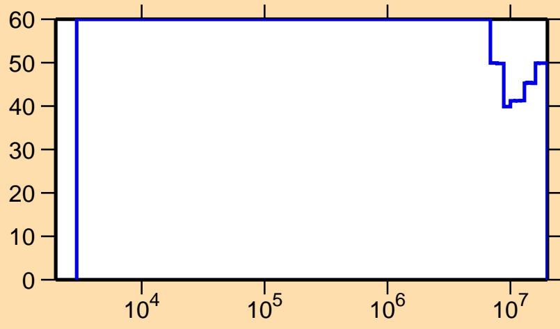
\Delta\sigma/\sigma vs. E for ^{60}\text{Cu}(n,\gamma)
