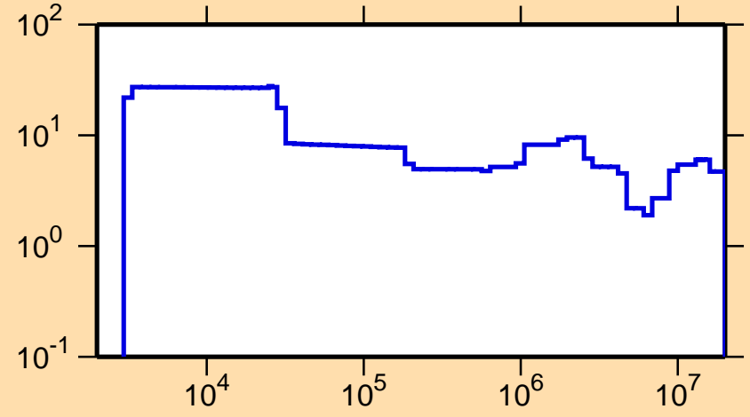
\Delta\sigma/\sigma vs. E for ^{60}\text{Cu}(n,\text{tot.})
