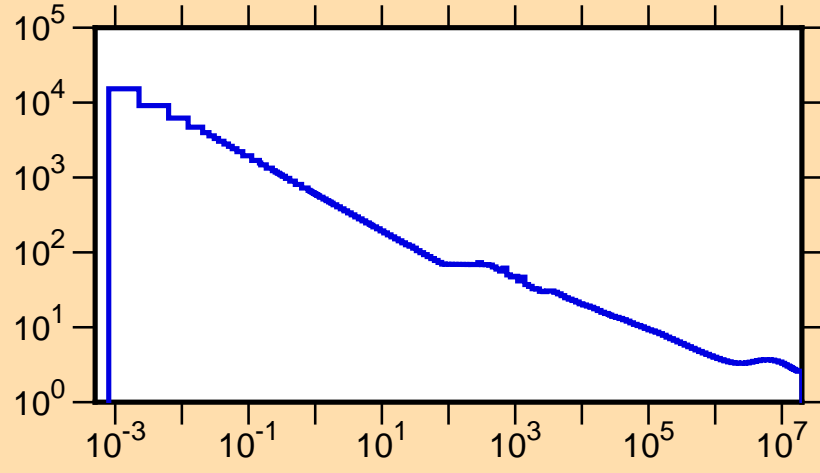
\sigma vs. E for ^{60}\text{Cu}(n,\text{tot.})
