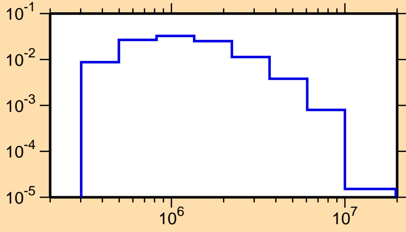
\sigma vs. E for ^{60}\text{Cu}(n,n_4)
