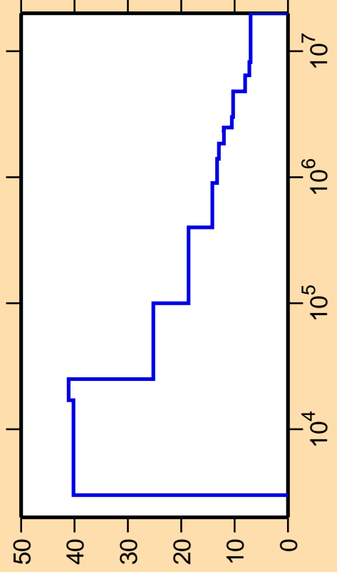
\Delta\sigma/\sigma vs. E for ^{60}\text{Cu}(n,\text{nonel.})
