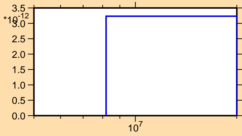
\sigma vs. E for ^{60}\text{Cu}(n,nt)
