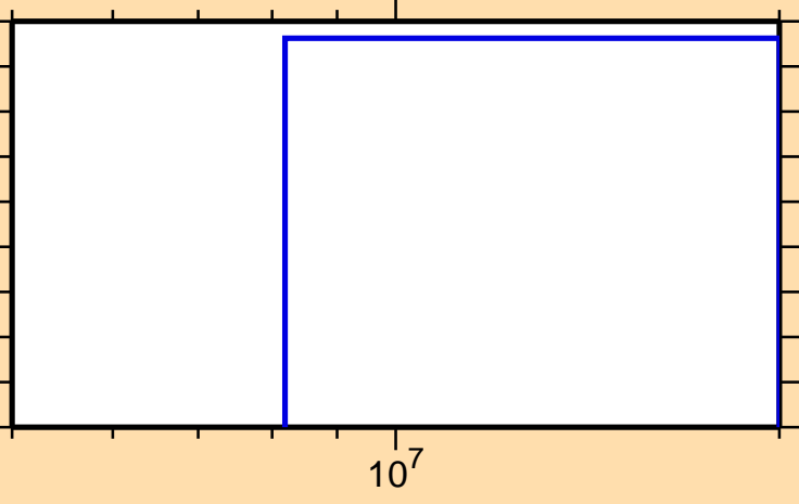
\sigma vs. E for ^{60}\text{Cu} (mt 45)
