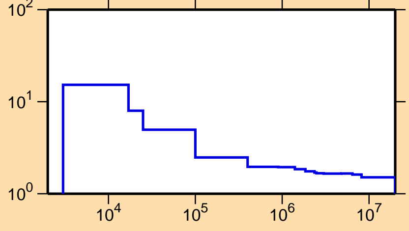
\sigma vs. E for ^{60}\text{Cu}(n,\text{nonel.})
