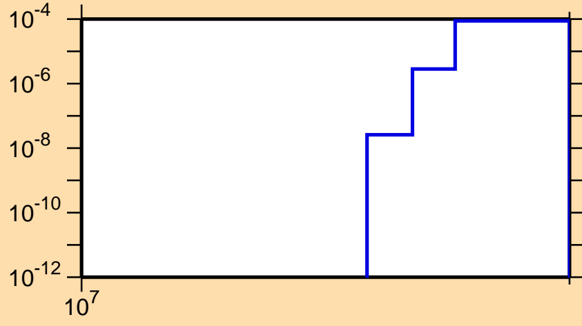
\sigma vs. E for ^{61}\text{Cu}(n,\text{nd})
