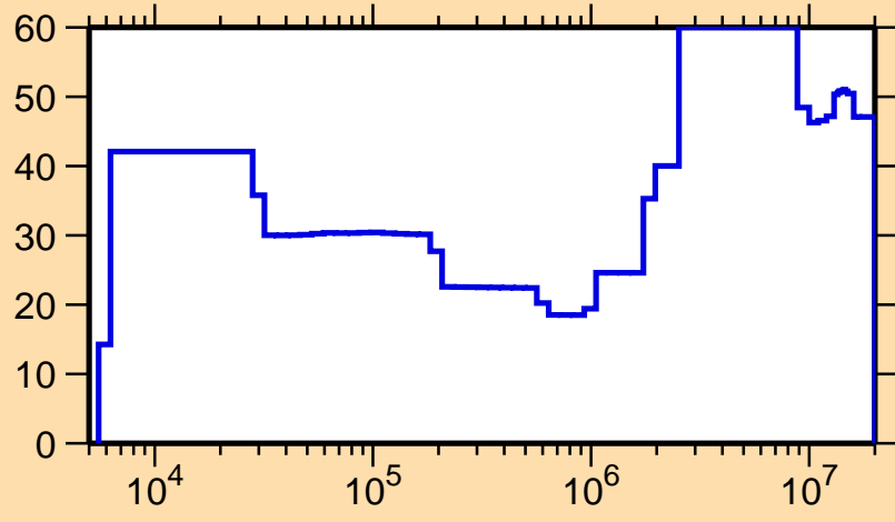
\Delta\sigma/\sigma vs. E for ^{61}\text{Cu}(n,p)
