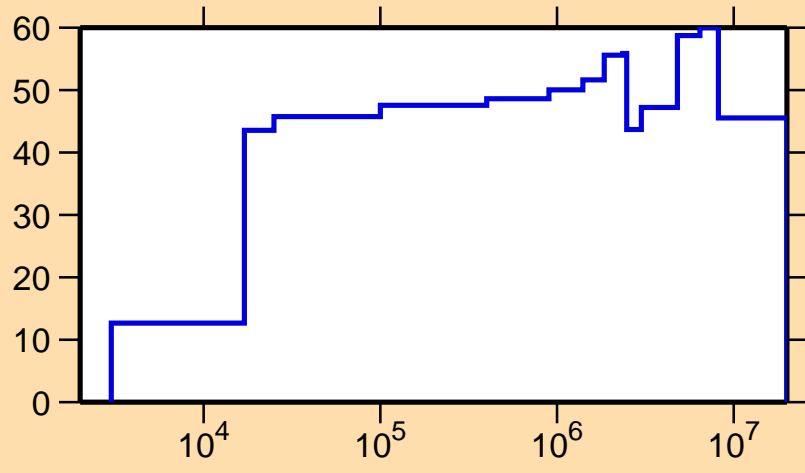
\Delta\sigma/\sigma vs. E for ^{61}\text{Cu}(n,\gamma)
