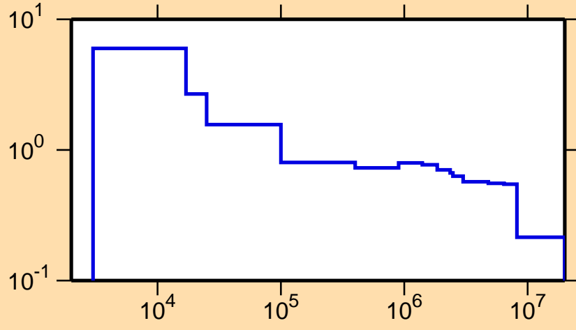
\sigma vs. E for ^{61}\text{Cu}(n,p)
