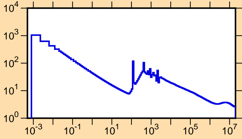
\sigma vs. E for ^{62}\text{Cu}(n,\text{tot.})
