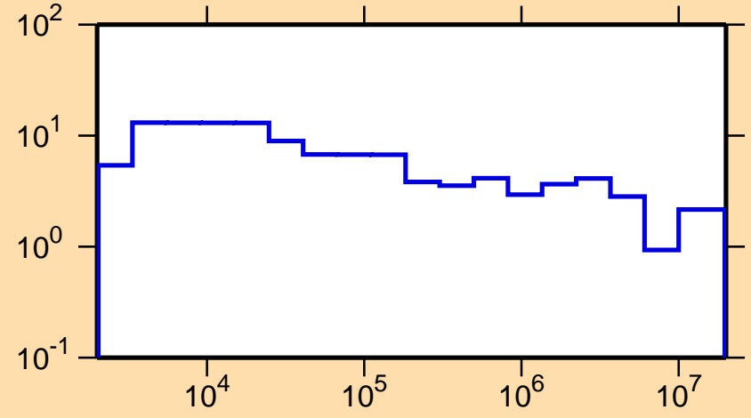
\Delta\sigma/\sigma vs. E for ^{62}\text{Cu}(n,\text{el.})
