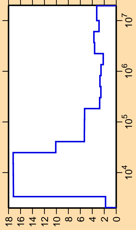
\Delta\sigma/\sigma vs. E for ^{62}\text{Cu}(n,\text{nonel.})
