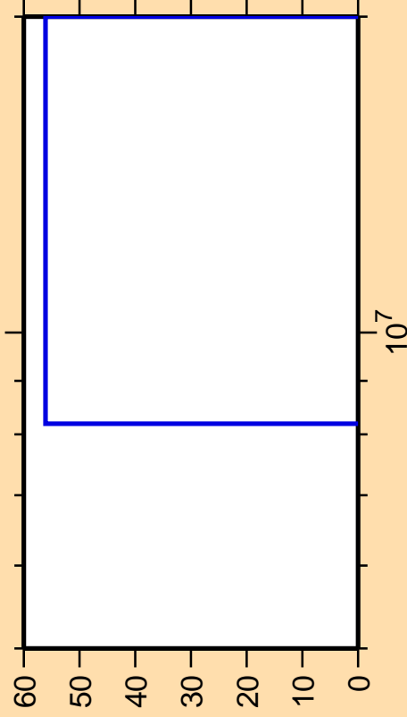
\Delta\sigma/\sigma vs. E for ^{62}\text{Cu}(n,nd)
