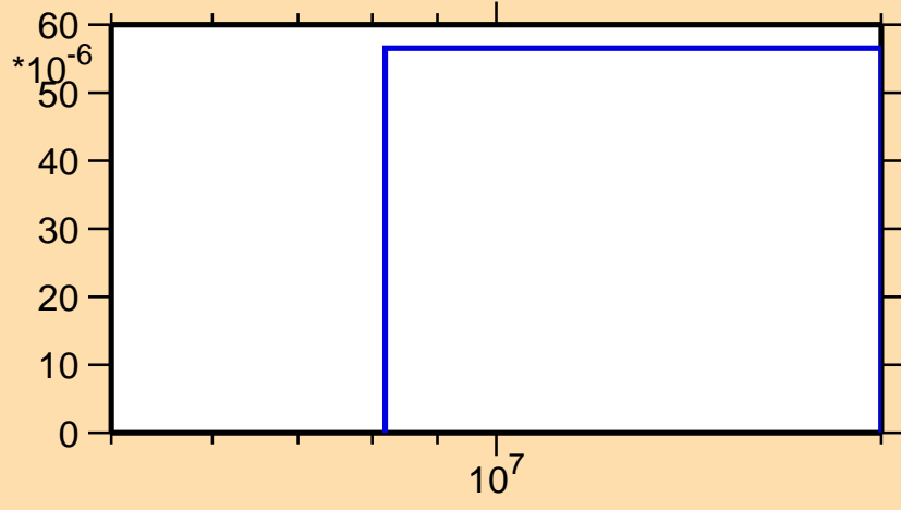
\sigma vs. E for ^{62}\text{Cu}(n,nd)
