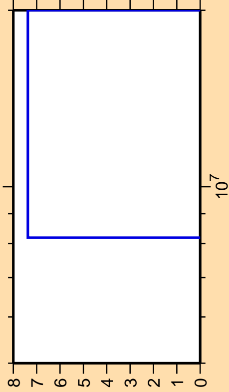
\Delta\sigma/\sigma vs. E for ^{62}\text{Cu}(n,n_1)
