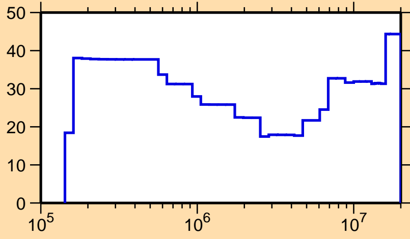
\Delta\sigma/\sigma vs. E for ^{63}\text{Cu}(n,p)
