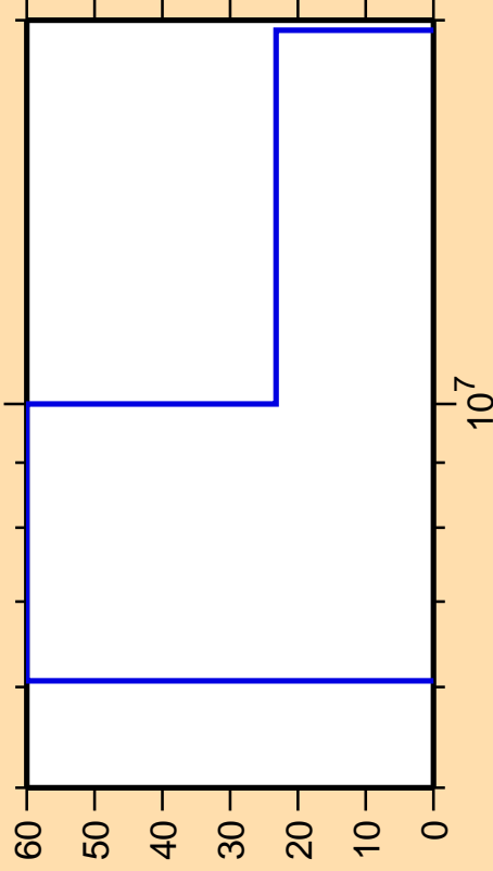
\Delta\sigma/\sigma vs. E for ^{63}\text{Cu}(n,n\alpha)
