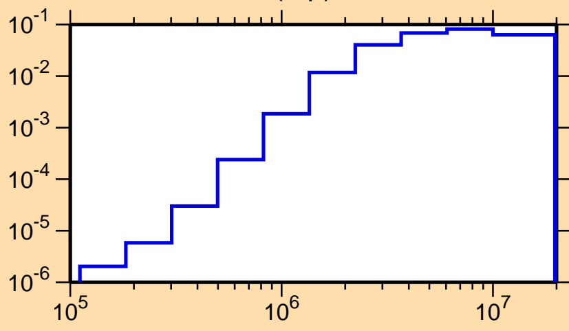
\sigma vs. E for ^{63}\text{Cu}(n,p)
