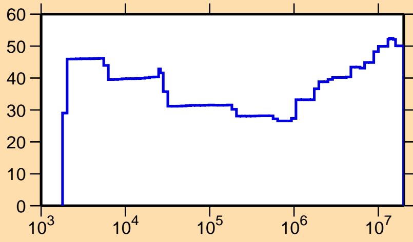
\Delta\sigma/\sigma vs. E for ^{64}\text{Cu}(n,p)
