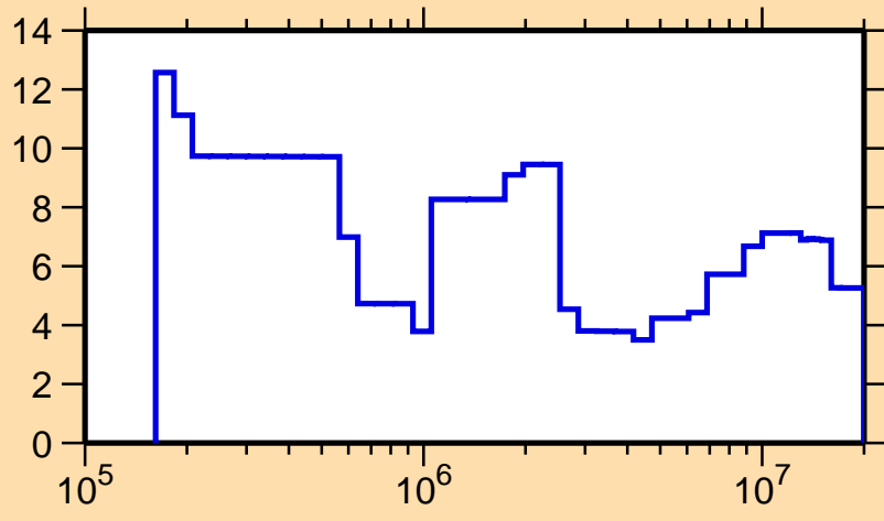
\Delta\sigma/\sigma vs. E for ^{64}\text{Cu}(n,\text{tot.})
