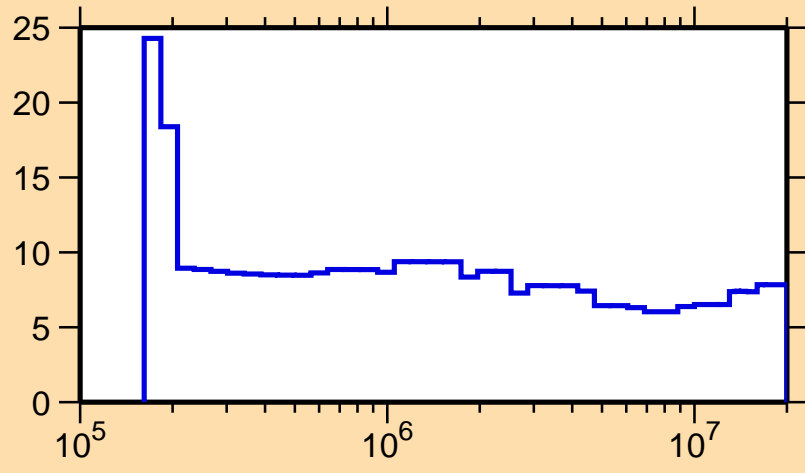
\Delta\sigma/\sigma vs. E for ^{64}\text{Cu}(n,\text{nonel.})
