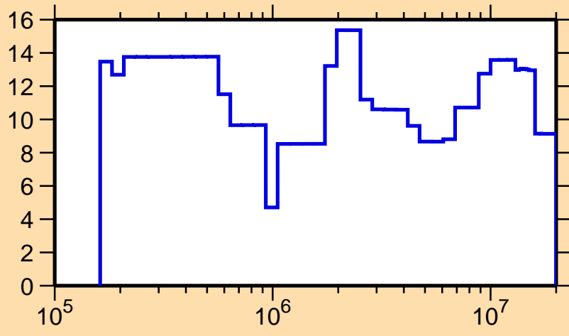
\Delta\sigma/\sigma vs. E for ^{64}\text{Cu}(n,\text{el.})
