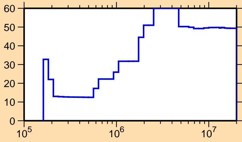
\Delta\sigma/\sigma vs. E for ^{64}\text{Cu}(n,n_1)
