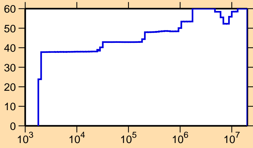
\Delta\sigma/\sigma vs. E for ^{64}\text{Cu}(n,\gamma)
