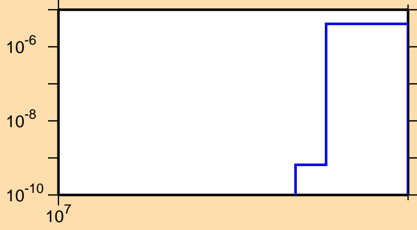
\sigma vs. E for ^{64}\text{Cu}(n,2n\alpha)
