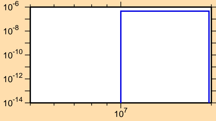
\sigma vs. E for ^{64}\text{Cu}(n,p\alpha)
