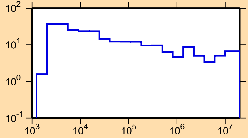
\Delta\sigma/\sigma vs. E for ^{64}\text{Cu}(n,\text{tot.})
