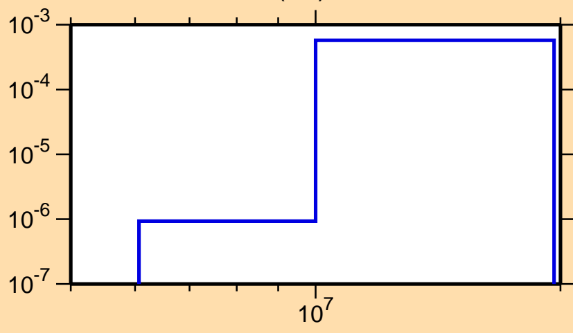
\sigma vs. E for ^{64}\text{Cu}(n,t)
