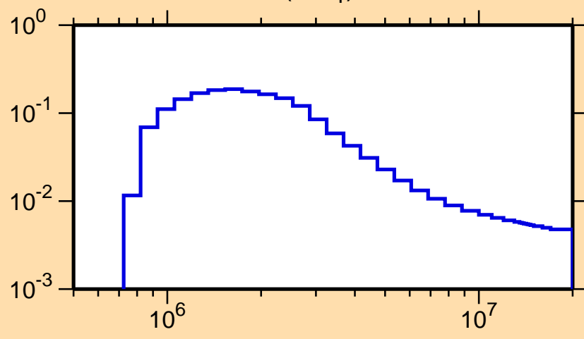
\sigma vs. E for ^{65}\text{Cu}(n,n_1)
