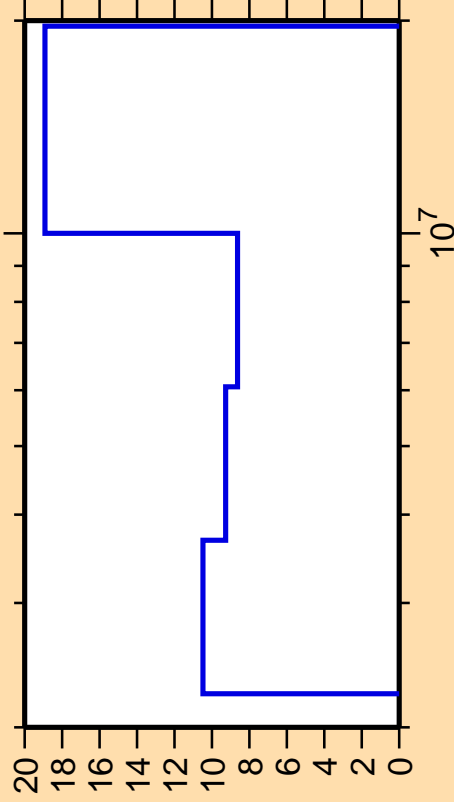
\Delta\sigma/\sigma vs. E for ^{65}\text{Cu}(n,n\text{cont.})
