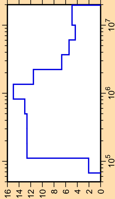
\Delta\sigma/\sigma vs. E for ^{65}\text{Cu}(n,\text{nonel.})
