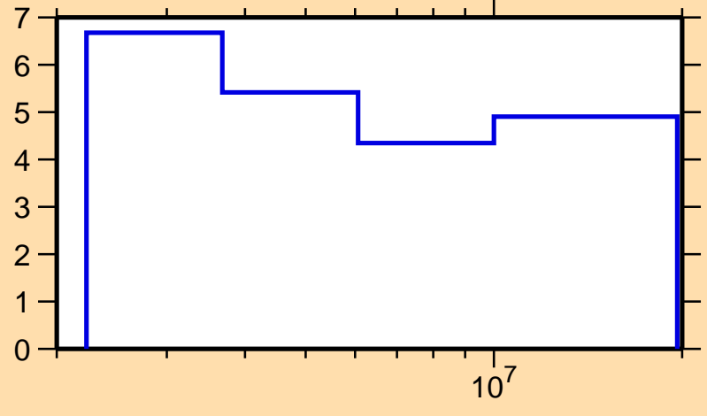
\Delta\sigma/\sigma vs. E for ^{65}\text{Cu}(n,n\text{nonel.})
