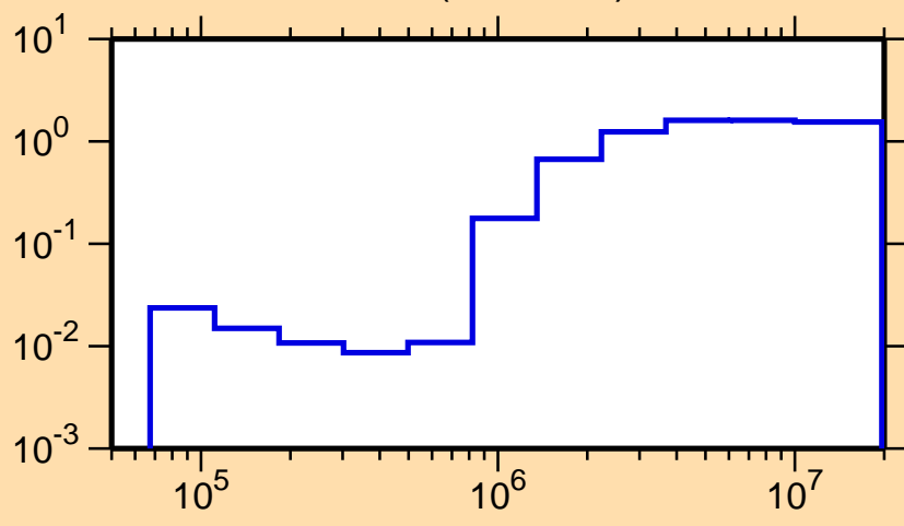
\sigma vs. E for ^{65}\text{Cu}(n,\text{nonel.})
