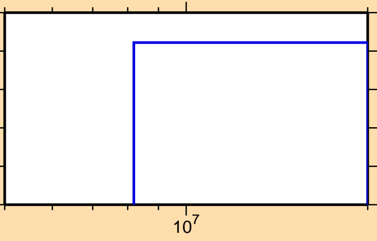
\sigma vs. E for ^{65}\text{Cu}(n,2np)
