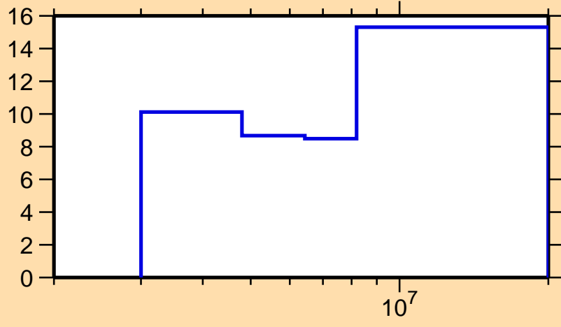
\Delta\sigma/\sigma vs. E for ^{65}\text{Cu}(n,ncont.)
