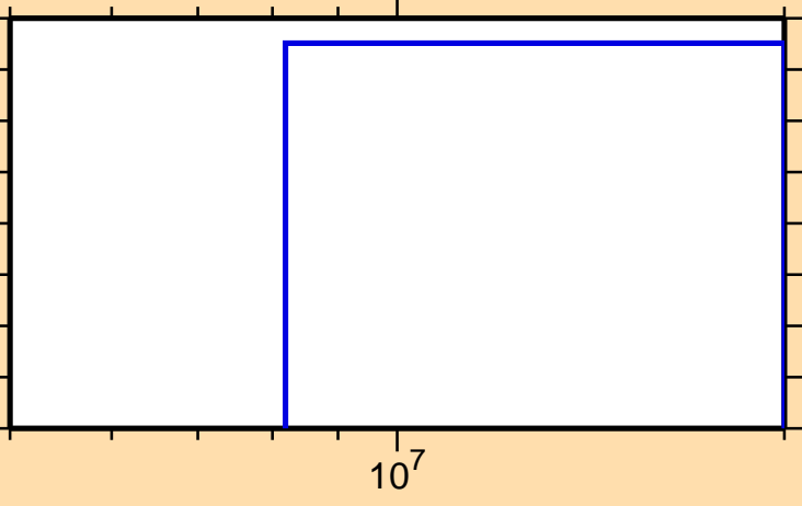
\sigma vs. E for ^{65}\text{Cu}(n,n\alpha)
