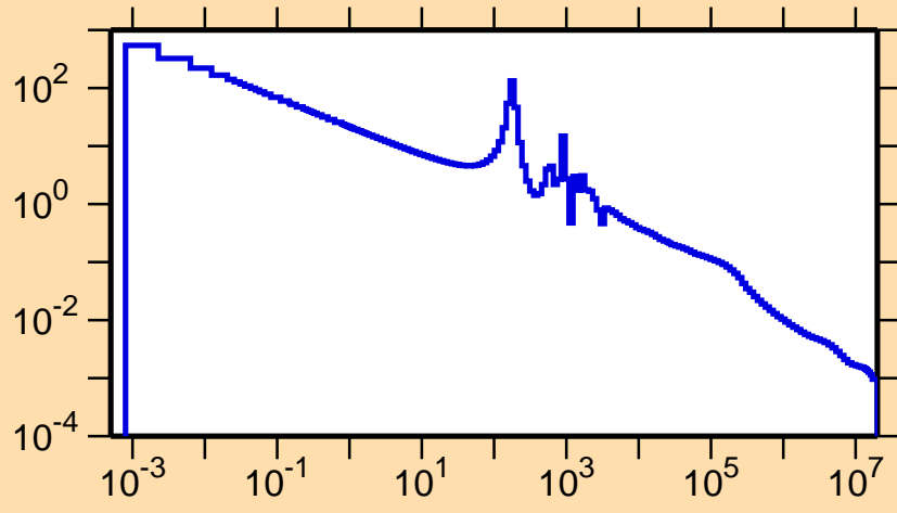
\sigma vs. E for ^{66}\text{Cu}(n,\gamma)
