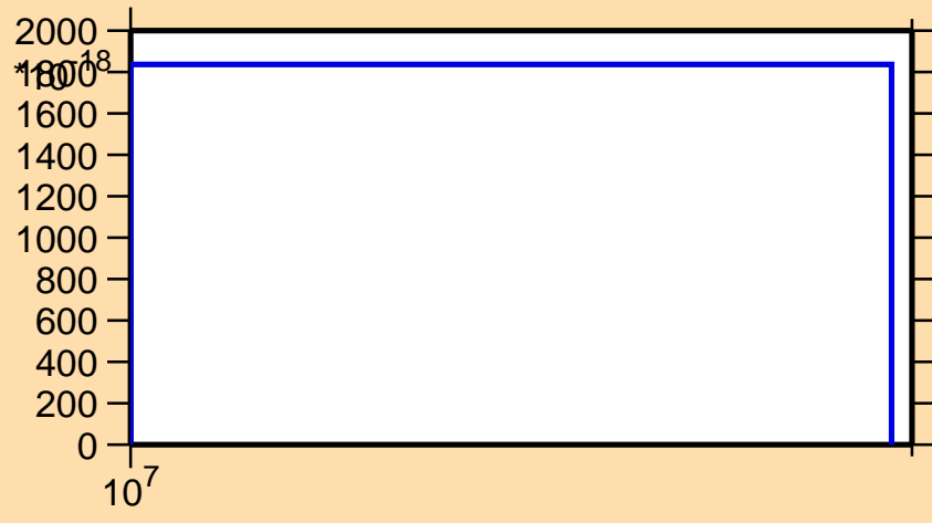
\sigma vs. E for ^{67}\text{Cu}(n,2n\alpha)
