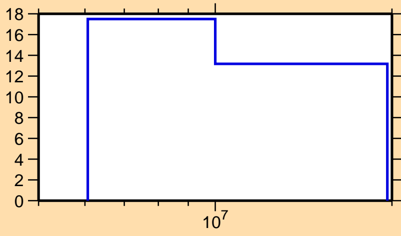
\Delta\sigma/\sigma vs. E for ^{67}\text{Cu}(n,2n)
