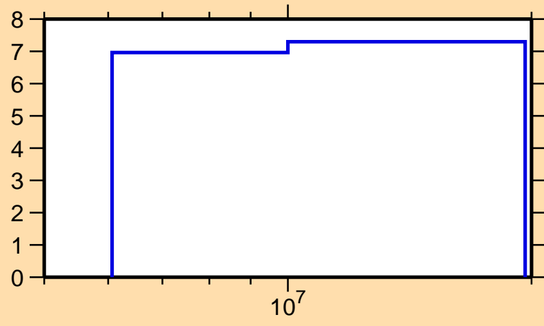
\Delta\sigma/\sigma vs. E for ^{67}\text{Cu}(n,\text{nonel.})
