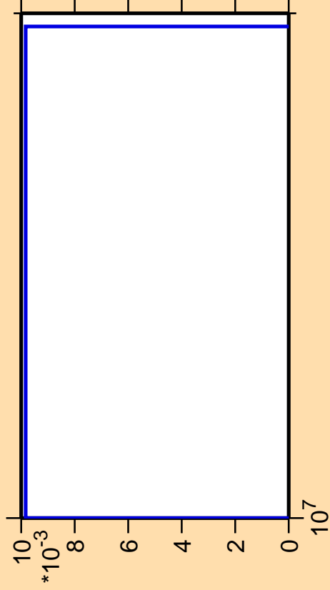
\Delta\sigma/\sigma vs. E for ^{67}\text{Cu}(n,2n\alpha)
