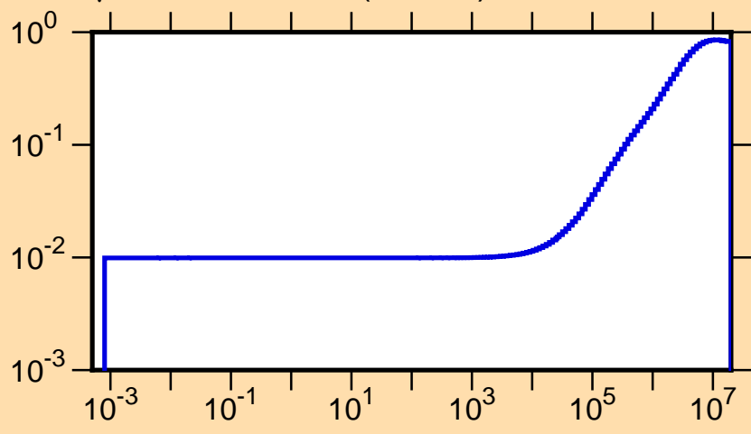
\mu vs. E for ^{68}\text{Cu}(\text{mt251})
