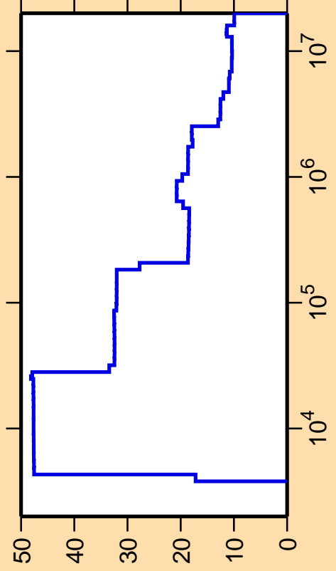
\Delta\sigma/\sigma vs. E for ^{68}\text{Cu}(n,\text{nonel.})
