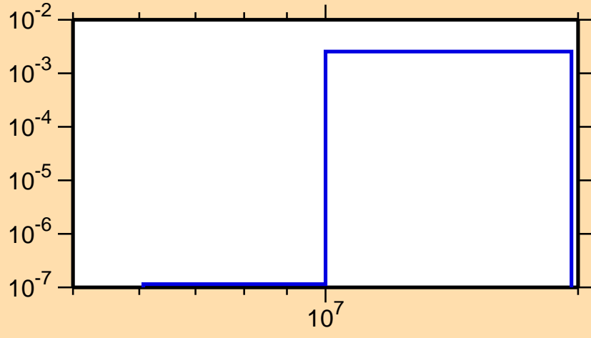
\sigma vs. E for ^{68}\text{Cu}(n,d)
