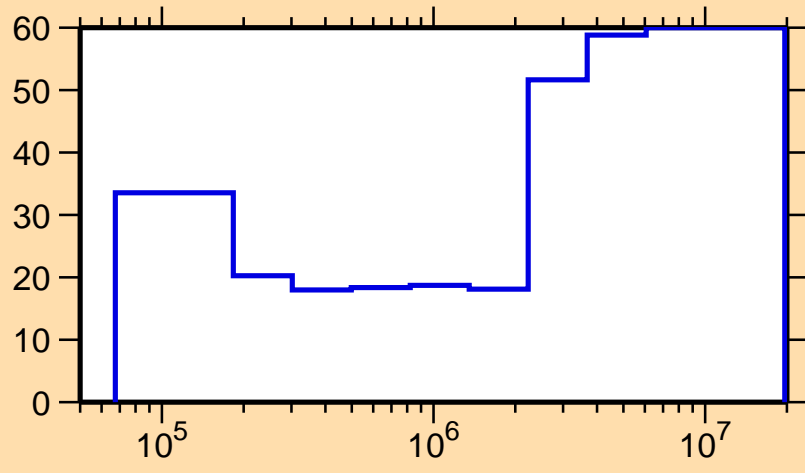
\Delta\sigma/\sigma vs. E for ^{68}\text{Cu}(n,n_1)
