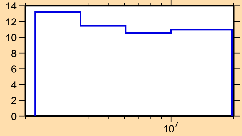
\Delta\sigma/\sigma vs. E for ^{68}\text{Cu}(n,n\text{nonel.})
