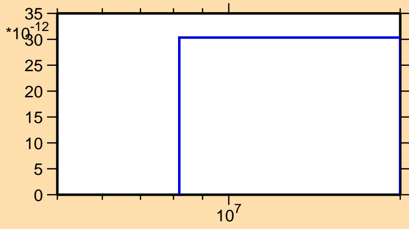
\sigma vs. E for ^{68}\text{Cu}(n,2n\alpha)
