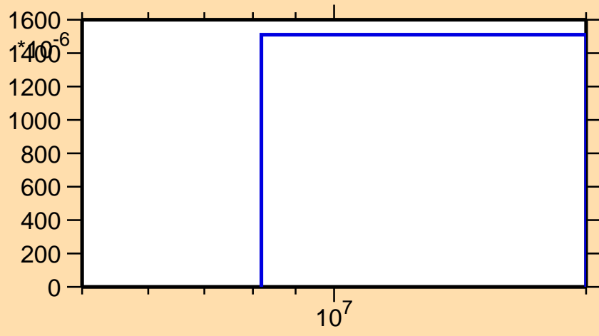
\sigma vs. E for ^{68}\text{Cu}(n,np)
