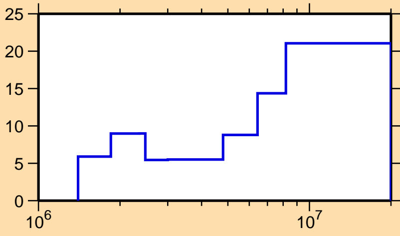
\Delta\sigma/\sigma vs. E for ^{68}\text{Cu}(n,el.)
