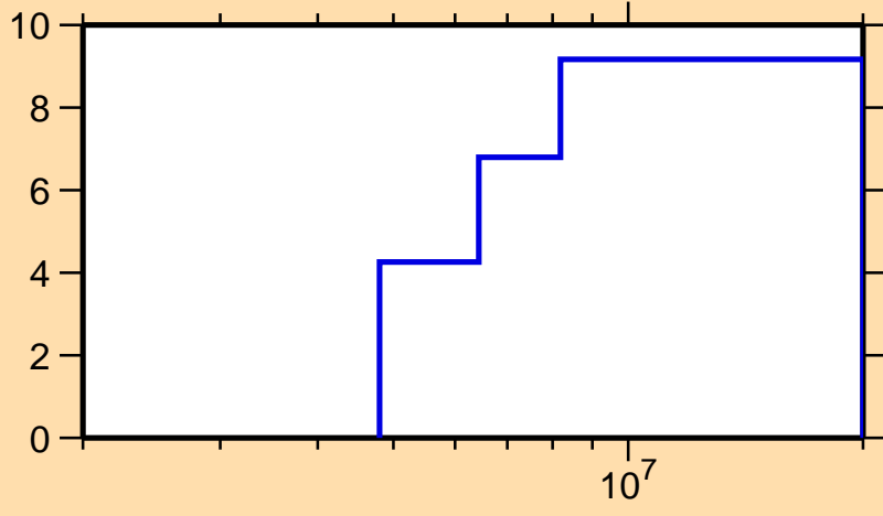
\Delta\sigma/\sigma vs. E for ^{68}\text{Cu}(n,\text{tot.})
