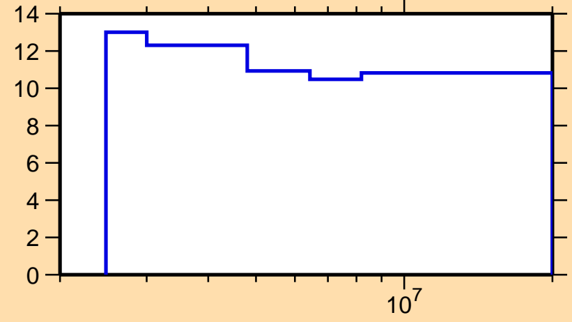
\Delta\sigma/\sigma vs. E for ^{68}\text{Cu}(n,n\text{onel.})
