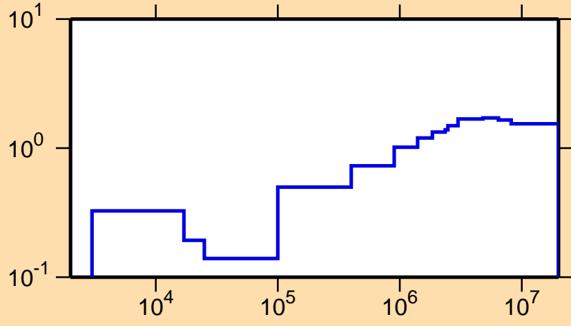
\sigma vs. E for ^{68}\text{Cu}(n,\text{nonel.})
