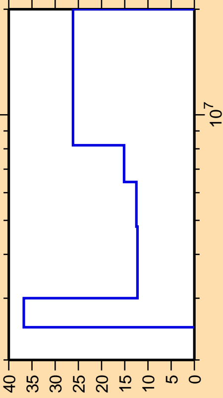
\sigma vs. E for ^{68}\text{Cu}(n,n\text{cont.})
