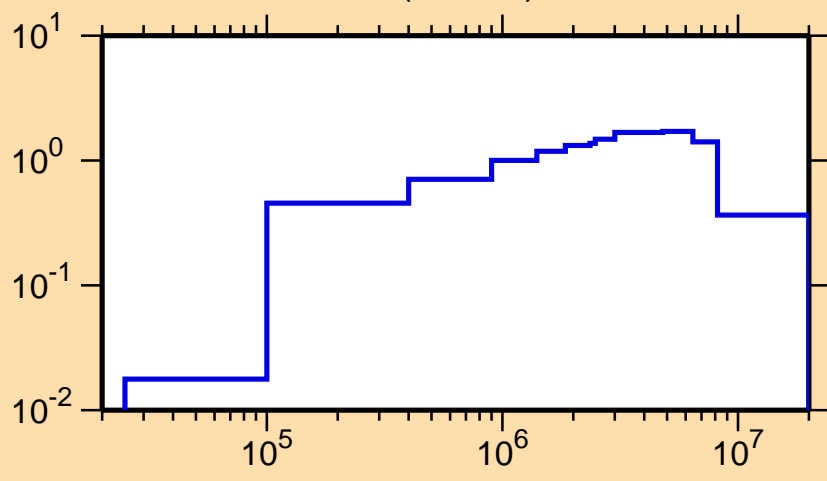
\sigma vs. E for ^{68}\text{Cu}(n,\text{inel.})
