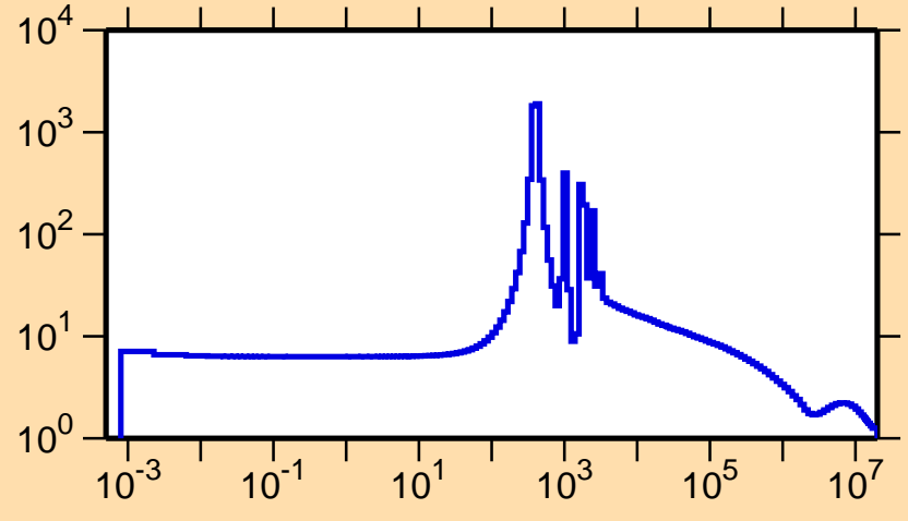
\sigma vs. E for ^{68}\text{Cu}(n,\text{el.})
