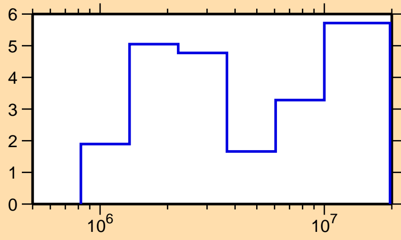
\Delta\sigma/\sigma vs. E for ^{68}\text{Cu}(n,el.)
