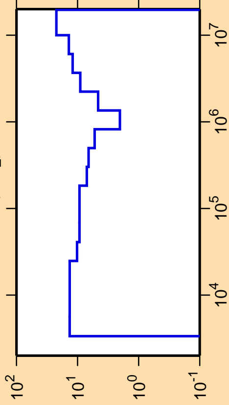
\Delta\sigma/\sigma vs. E for ^{68}\text{Cu}(n,n_2)
