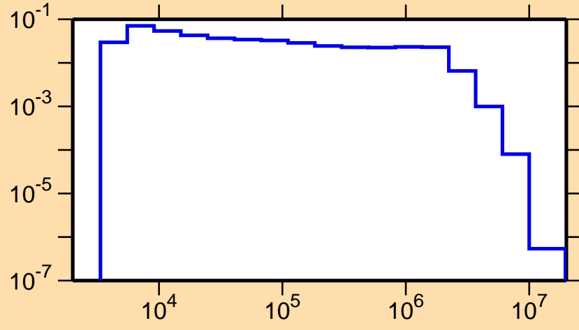
\sigma vs. E for ^{68}\text{Cu}(n,n_2)
