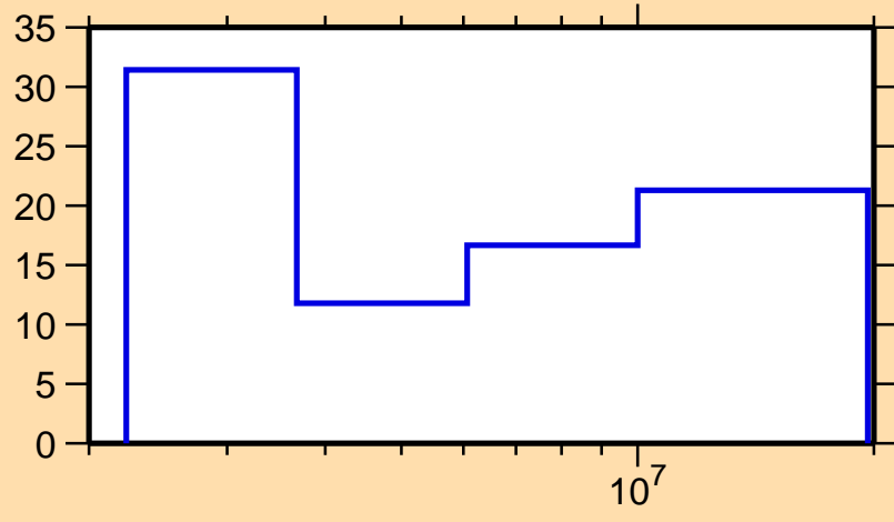
\Delta\sigma/\sigma vs. E for ^{68}\text{Cu}(n,p)
