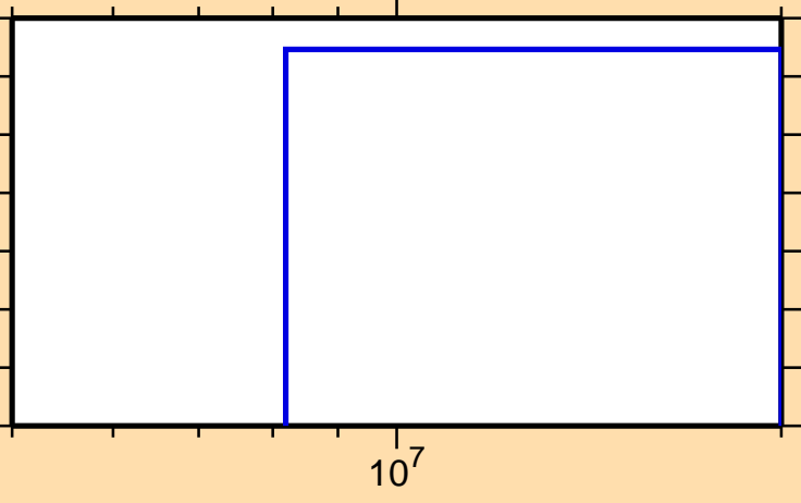
\sigma vs. E for ^{68}\text{Cu}(n,nt)
