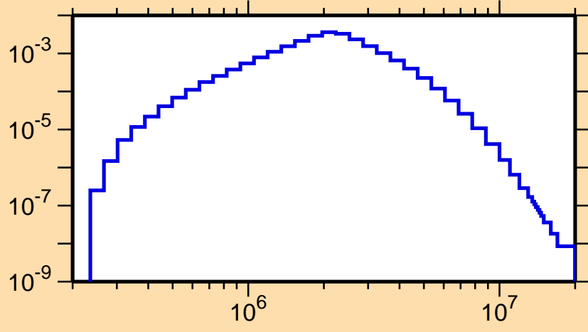
\sigma vs. E for ^{70}\text{Cu}(n,n_3)
