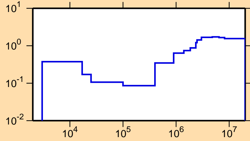
\sigma vs. E for ^{70}\text{Cu}(n,\text{nonel.})
