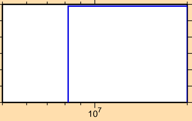
\sigma vs. E for ^{70}\text{Cu}(n,3n)
