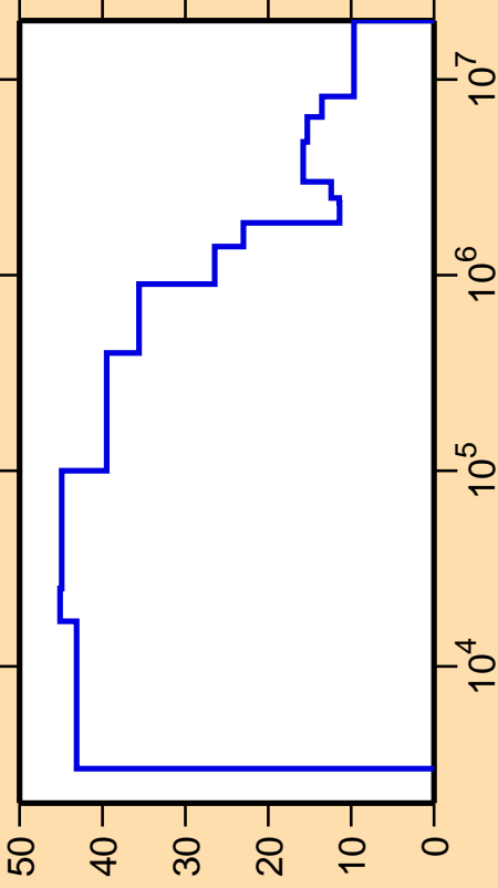
\Delta\sigma/\sigma vs. E for ^{70}\text{Cu}(n,\text{nonel.})
