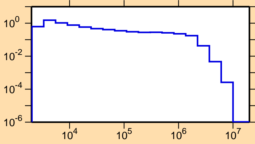
\sigma vs. E for ^{70}\text{Cu}(n,n_2)
