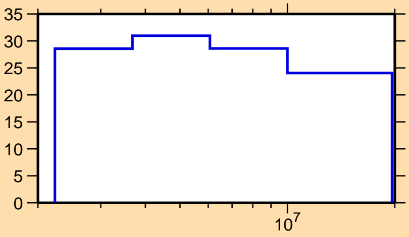
\Delta\sigma/\sigma vs. E for ^{71}\text{Cu}(n,n\text{nonel.})
