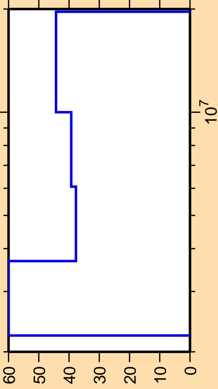
\Delta\sigma/\sigma vs. E for ^{71}\text{Cu}(n,n\text{cont.})
