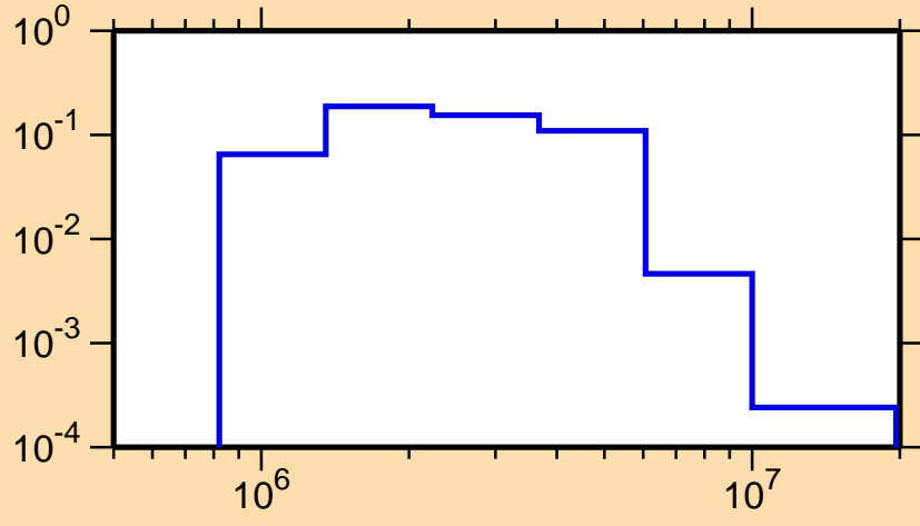
\sigma vs. E for ^{71}\text{Cu}(n,n_3)
