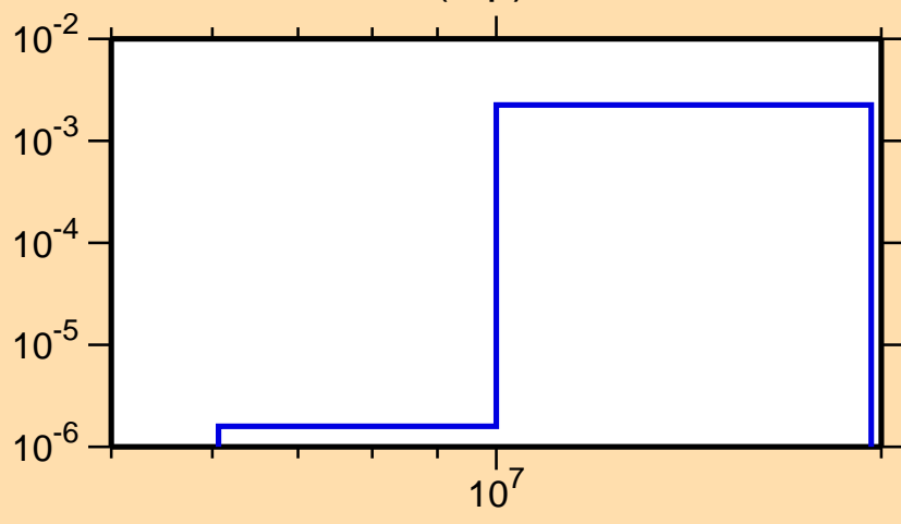
\sigma vs. E for ^{71}\text{Cu}(n,p)
