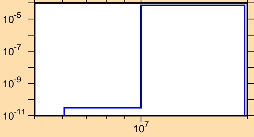
\sigma vs. E for ^{71}\text{Cu}(n,\alpha)
