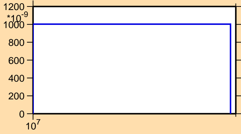
\sigma vs. E for ^{71}\text{Cu}(n,n\alpha)
