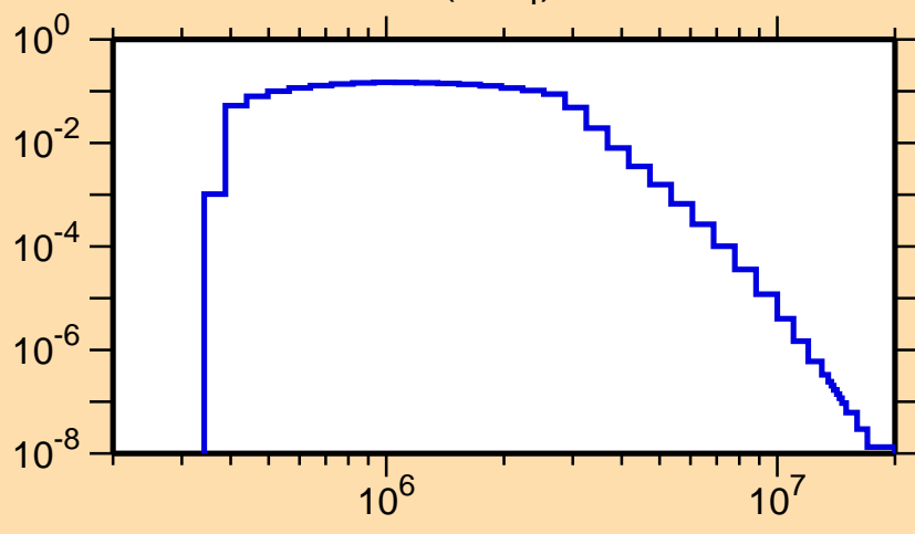
\sigma vs. E for ^{72}\text{Cu}(n,n_4)
