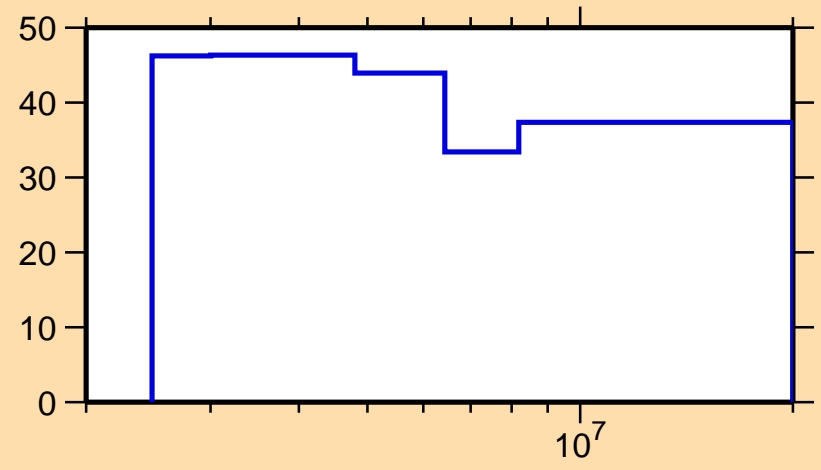
\Delta\sigma/\sigma vs. E for ^{72}\text{Cu}(n,n\text{nonel.})
