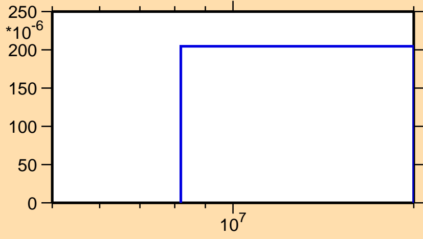
\sigma vs. E for ^{72}\text{Cu}(n,d)
