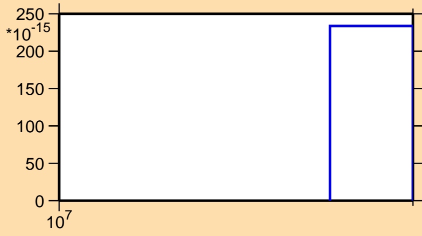
\sigma vs. E for ^{73}\text{Cu}(n,2np)
