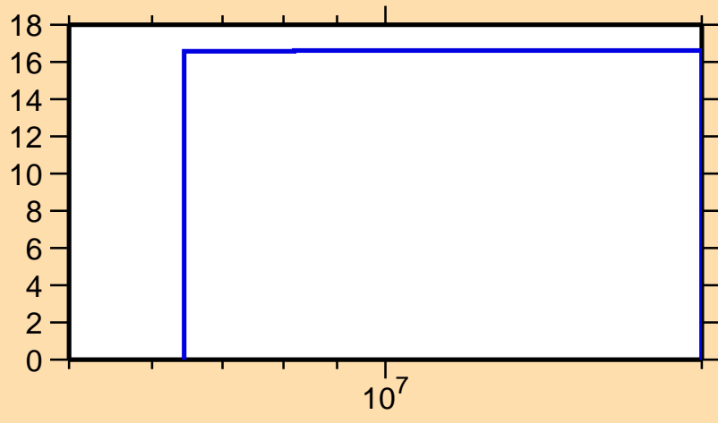
\Delta\sigma/\sigma vs. E for ^{73}\text{Cu}(n,\text{tot.})
