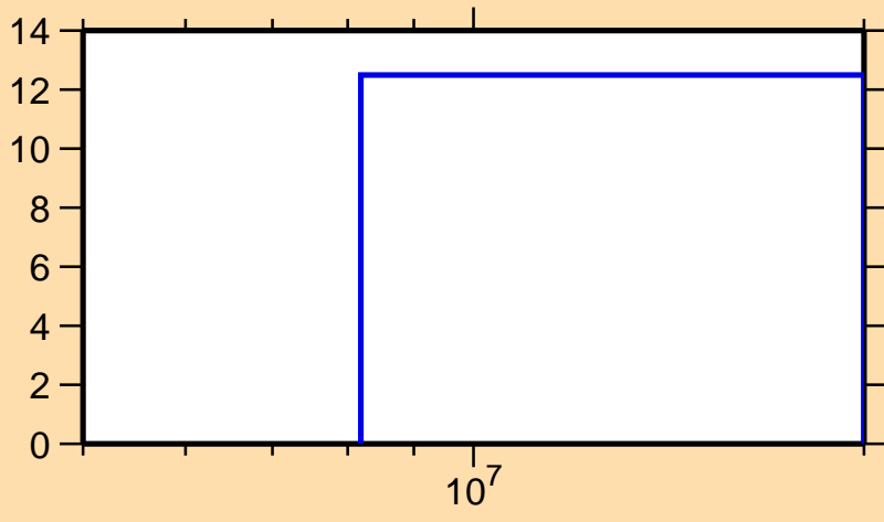
\Delta\sigma/\sigma vs. E for ^{73}\text{Cu}(n,\text{nonel.})
