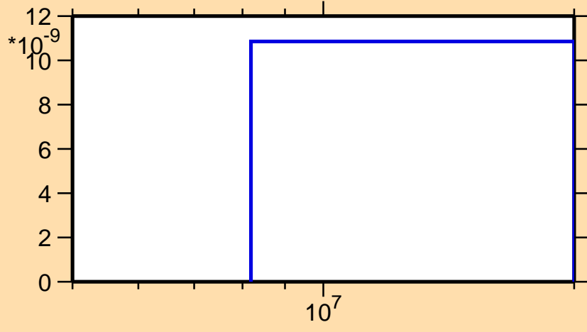
\sigma vs. E for ^{73}\text{Cu}(n,nt)
