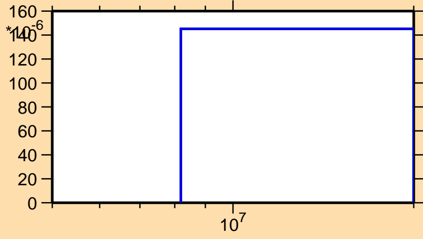
\sigma vs. E for ^{73}\text{Cu}(n,d)
