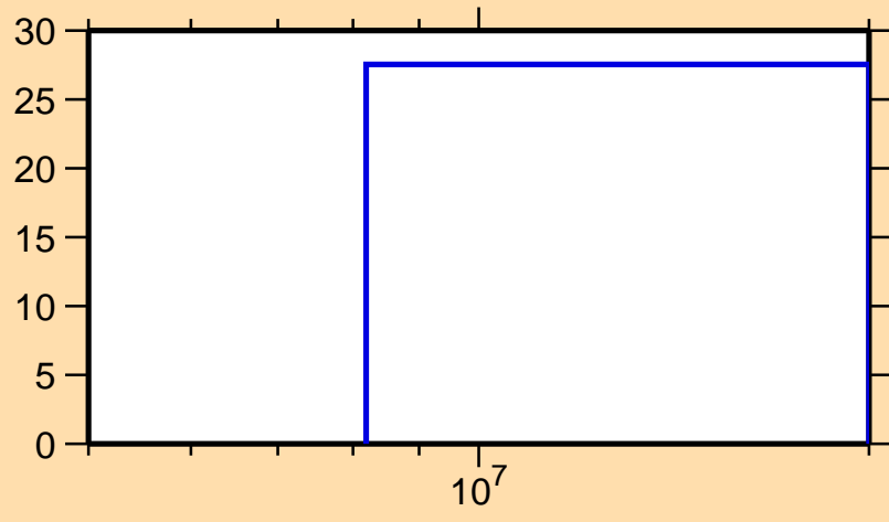
\Delta\sigma/\sigma vs. E for ^{73}\text{Cu}(n,el.)
