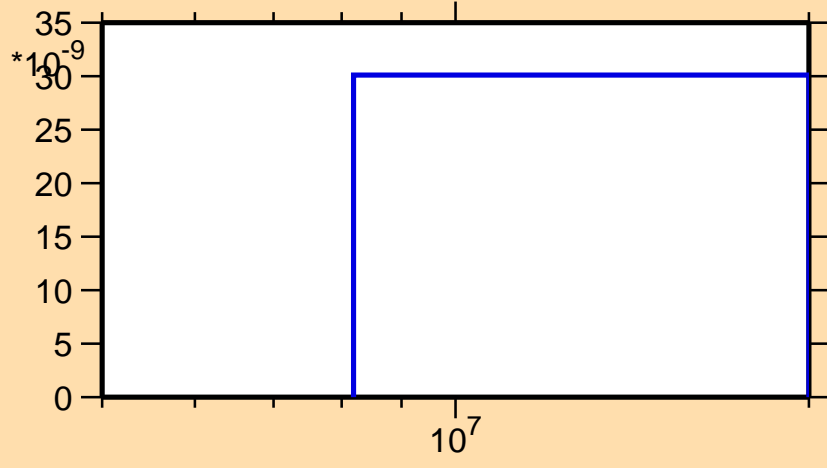
\sigma vs. E for ^{73}\text{Cu}(n,n\alpha)
