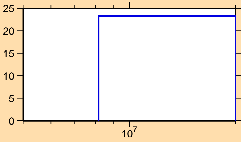
\Delta\sigma/\sigma vs. E for ^{73}\text{Cu}(n,2n)
