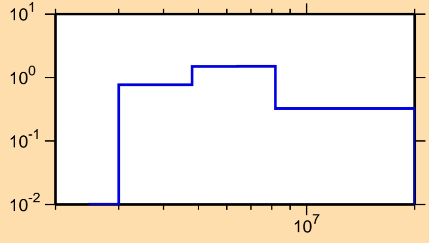
\sigma vs. E for ^{73}\text{Cu}(n,n\text{cont.})
