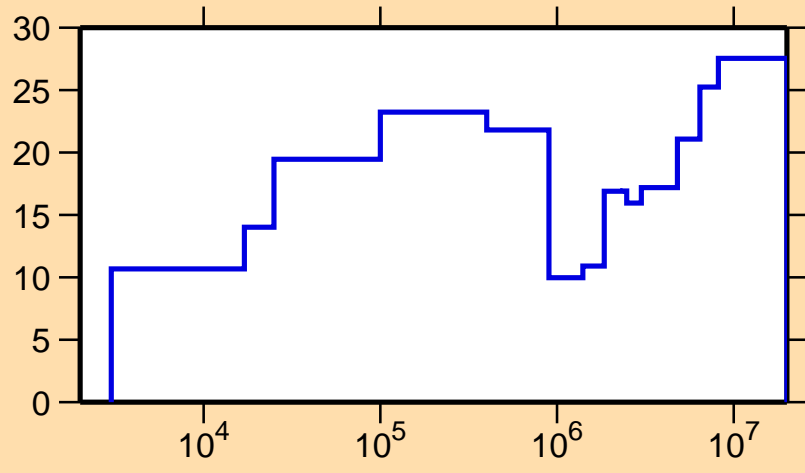
\Delta\sigma/\sigma vs. E for ^{73}\text{Cu}(n,\text{el.})
