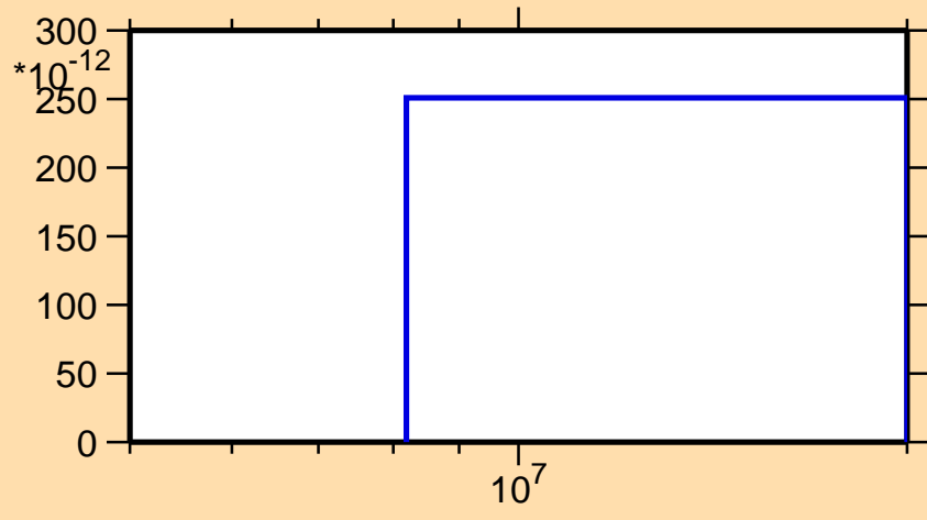
\sigma vs. E for ^{73}\text{Cu}(n,\text{nd})
