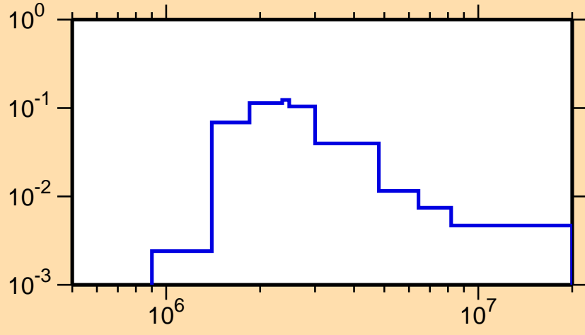
\sigma vs. E for ^{73}\text{Cu}(n,n_4)
