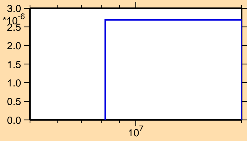
\sigma vs. E for ^{73}\text{Cu}(n,t)
