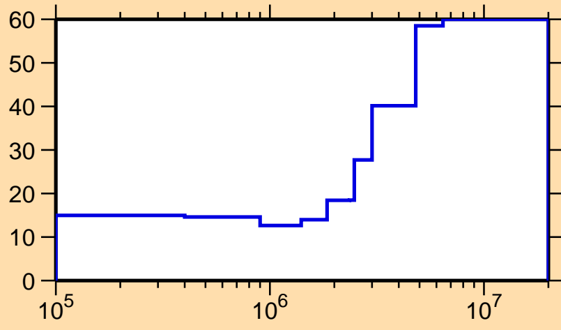
\Delta\sigma/\sigma vs. E for ^{73}\text{Cu}(n,n_1)
