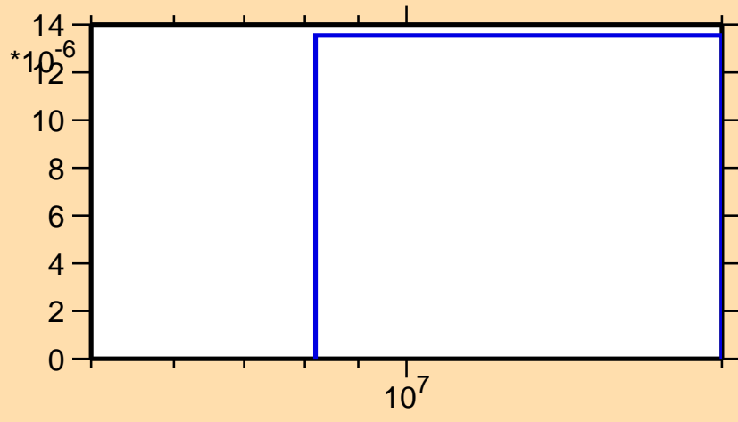
\sigma vs. E for ^{73}\text{Cu}(n,np)
