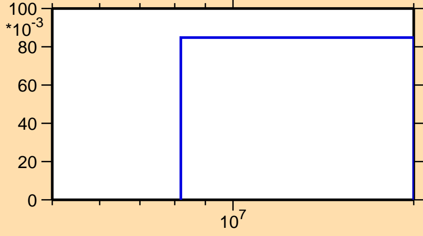
\sigma vs. E for ^{73}\text{Cu}(n,3n)
