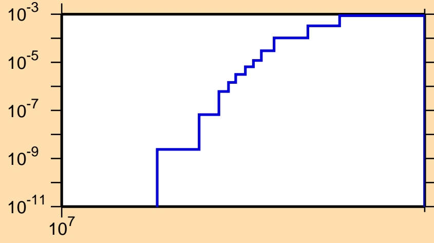
\sigma vs. E for ^{74}\text{Cu}(n,d)
