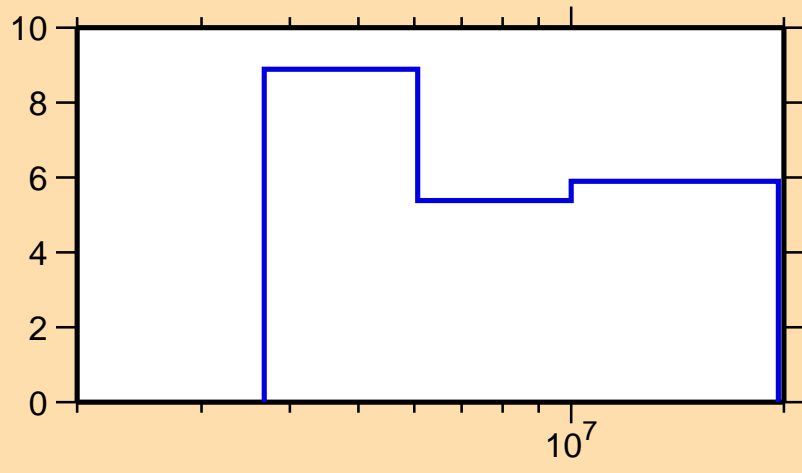
\Delta\sigma/\sigma vs. E for ^{74}\text{Cu}(n,\text{nonel.})
