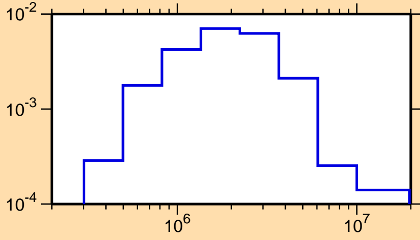
\sigma vs. E for ^{74}\text{Cu}(n,n_1)
