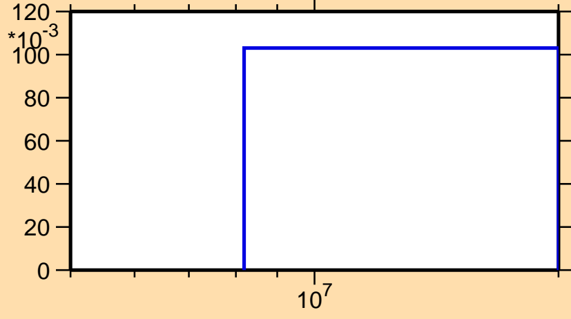
\sigma vs. E for ^{74}\text{Cu}(n,3n)
