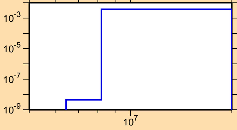
\sigma vs. E for ^{74}\text{Cu}(n,p)
