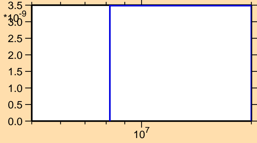
\sigma vs. E for ^{74}\text{Cu}(n,nt)
