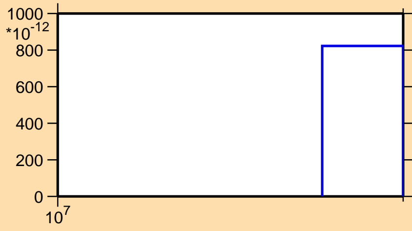
\sigma vs. E for ^{75}\text{Cu}(n,\text{nd})
