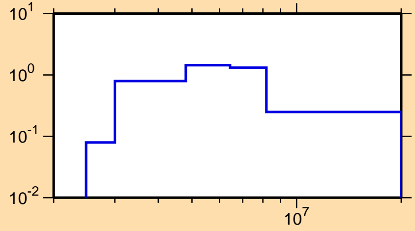
\sigma vs. E for ^{75}\text{Cu}(n,n\text{cont.})
