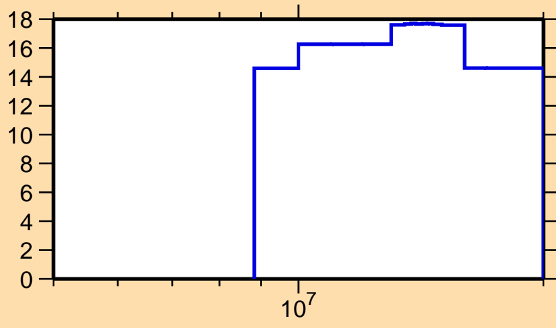
\Delta\sigma/\sigma vs. E for ^{76}\text{Cu}(n,el.)
