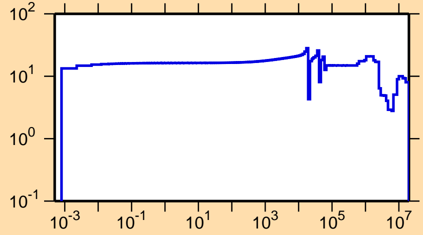
\Delta\sigma/\sigma vs. E for ^{76}\text{Cu}(n,\text{tot.})
