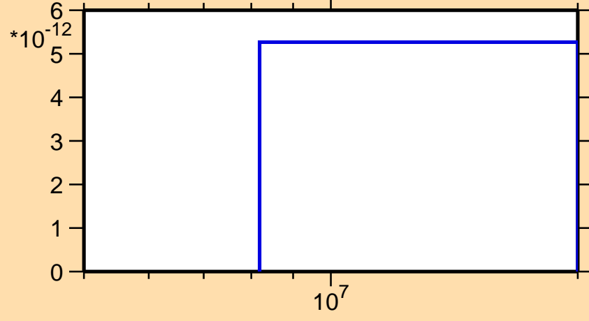
\sigma vs. E for ^{76}\text{Cu}(n,2np)
