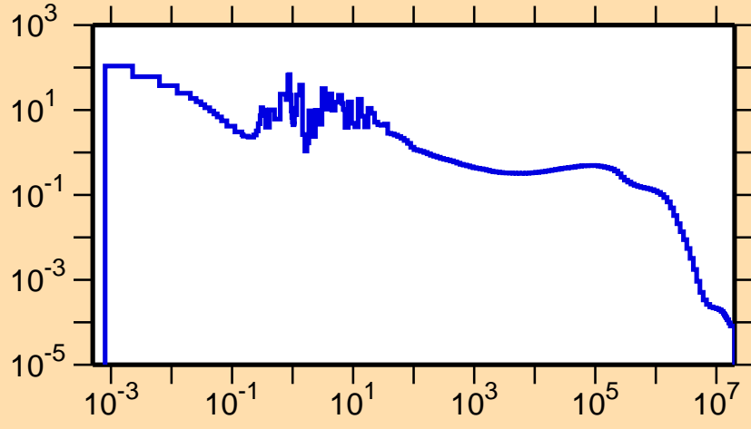
\sigma vs. E for ^{255}\gamma
