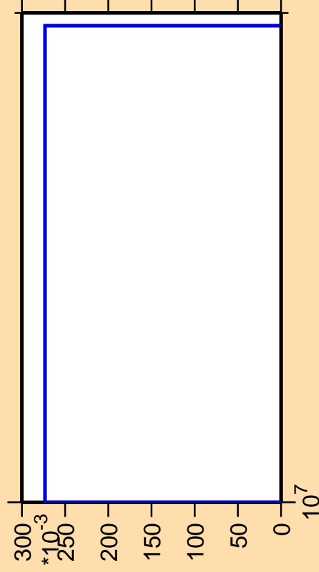
\Delta\sigma/\sigma vs. E for ^{255}
