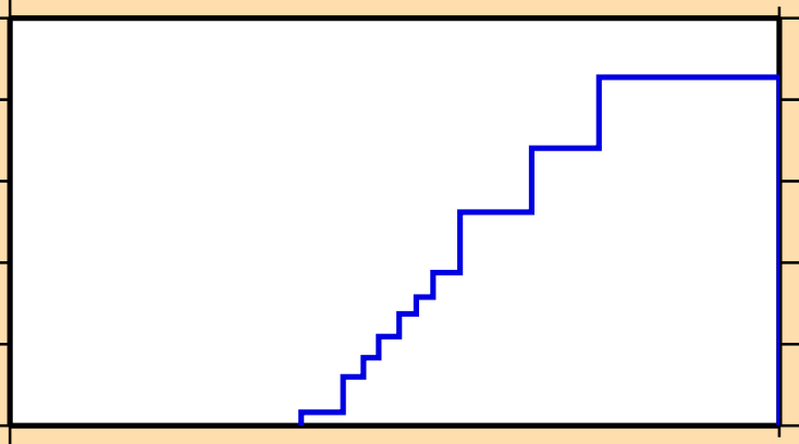
\sigma vs. E for ^{256}
