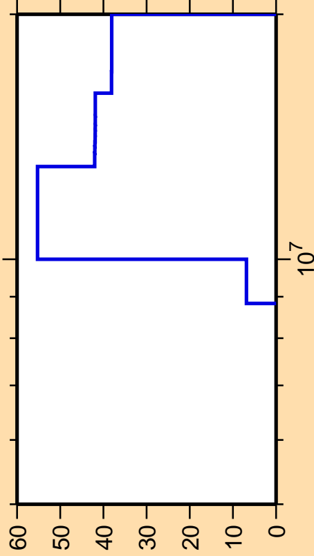
\Delta\sigma/\sigma vs. E for ^{256}\text{He3}
