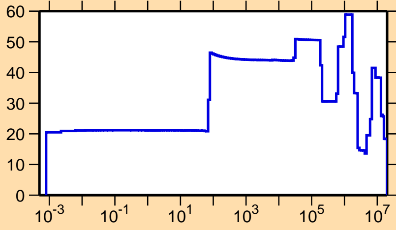
\Delta\sigma/\sigma vs. E for ^{256}\text{Ge}
