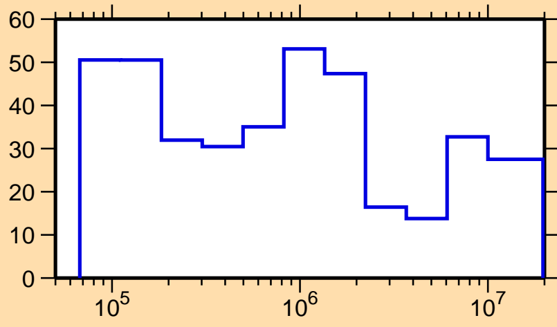
Δσ/σ vs. E for 256
