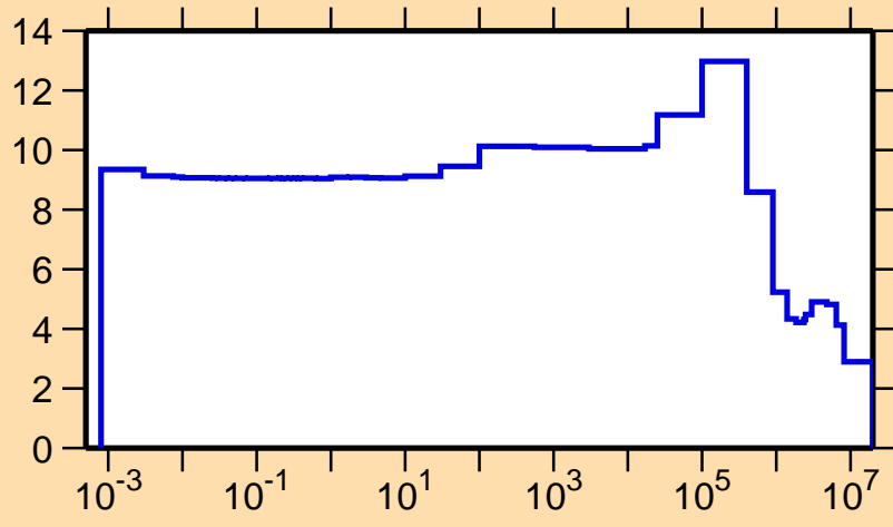
\sigma vs. E for ^{256}
