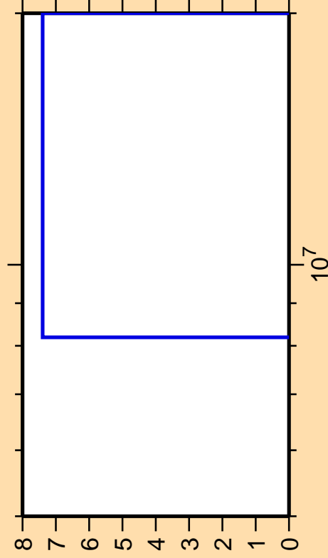
\Delta\sigma/\sigma vs. E for 256
