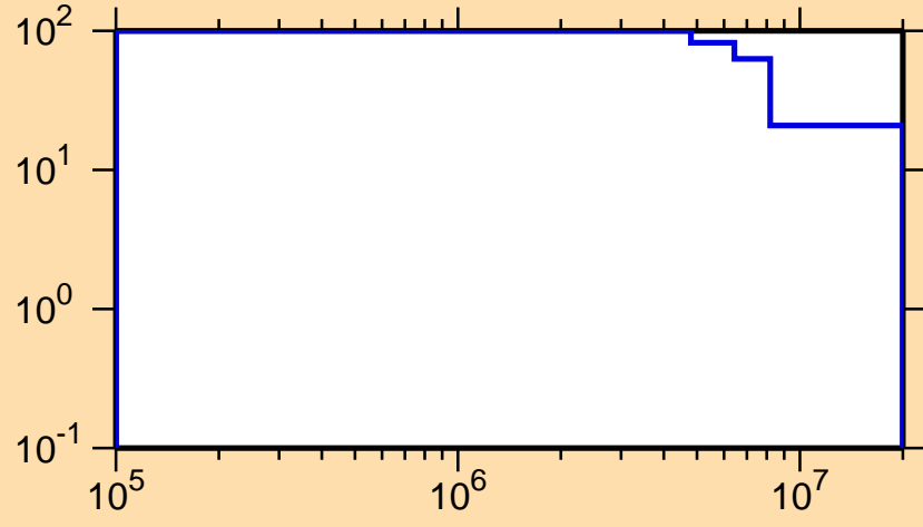
\Delta\sigma/\sigma vs. E for ^{256}\text{Po}
