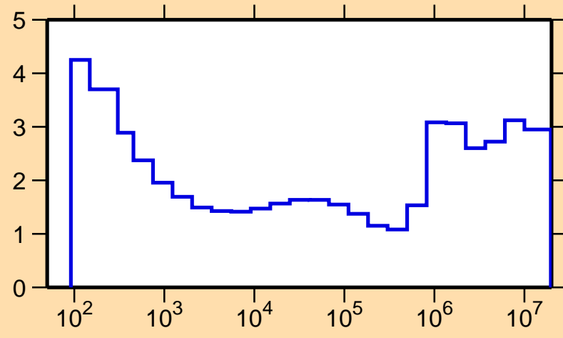
\sigma vs. E for ^{257}
